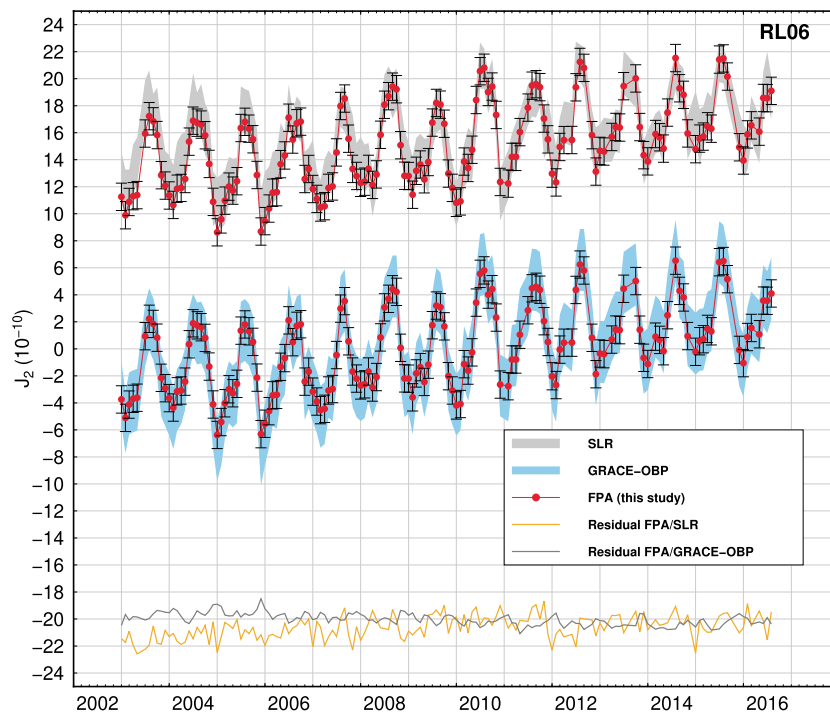
Figure 2. A comparison of J_2 estimates obtained from CSR RL06 data using the FPA approach (this study; red curve with dots) with those obtained using the GRACE-OBP approach (Sun et al., 2016; blue band), as well as with those based on SLR data (Cheng et al., 2013; gray band). An offset of (15 \times 10^{-10}) is applied to the top pair of curves. Note that the SLR solution is represented by a gray band where the upper and lower bounds are defined by the \mu \pm 2\sigma ( \mu denotes the mean values), respectively. The same is also applied to the GRACE-OBP solution, where the uncertainty ( \sigma = 1.13 \times 10^{-10} ) is calculated based on Ditmar et al. (2018). The error bars are also shown for the FPA solution. All three solutions represent the full J_2 signals, which means that the J_2 contributions from the atmosphere and dynamic ocean effects have been restored in the GRACE-based solutions. The differences between FPA and SLR as well as between FPA and GRACE-OBP are shown at the bottom of the plot with an offset of -20 \times 10^{-10} being applied for clarity. The time series are based on the RL06 solutions, meaning that AOD RL06 product is adopted; the SLR solution uses AOD RL06 as background model. A RL05 version is available in the supporting information (Figure S9). CSR = Center for Space Research; FPA = fingerprint approach; GRACE = Gravity Recovery And Climate Experiment; OBP = ocean bottom pressure; SLR = satellite laser ranging.
